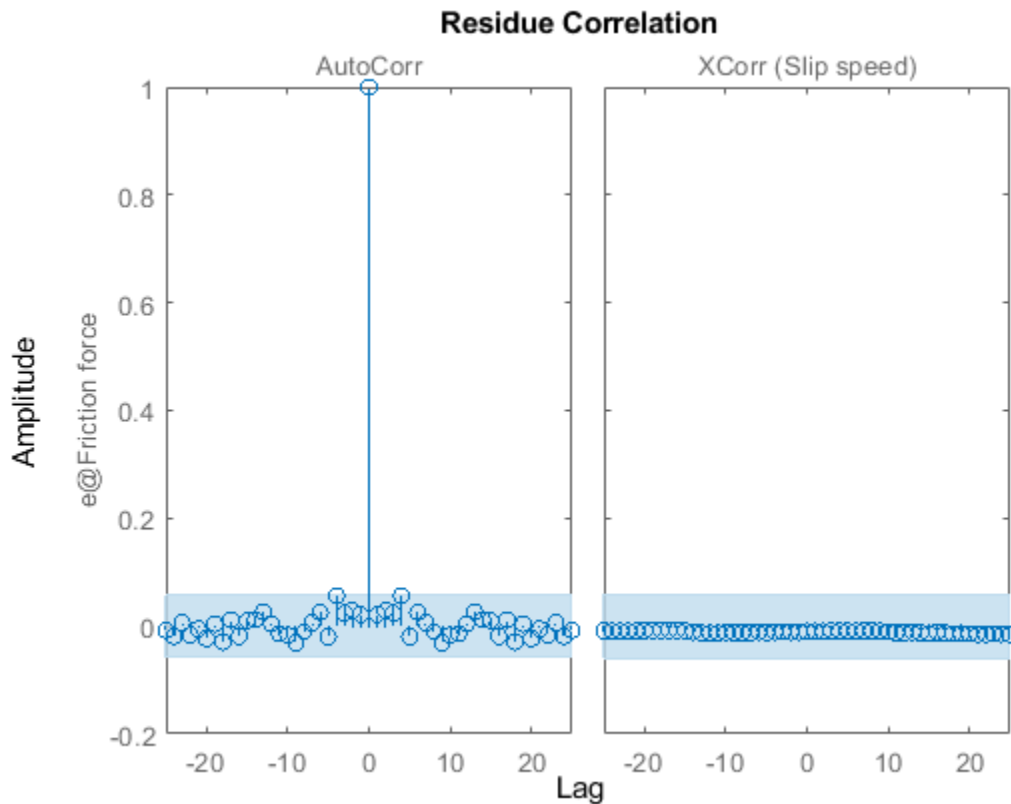
Figure 5: Residuals obtained with the estimated full friction model.
