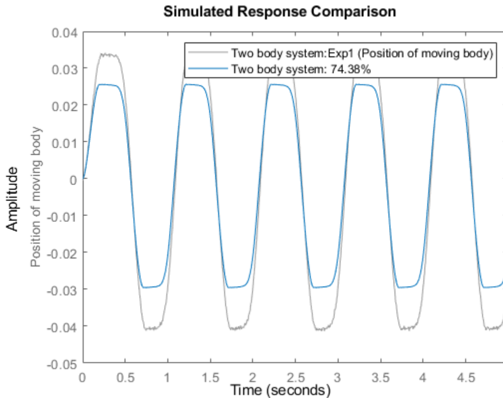
Figure 3: Comparison between true outputs and the simulated outputs of the initial two body model.
