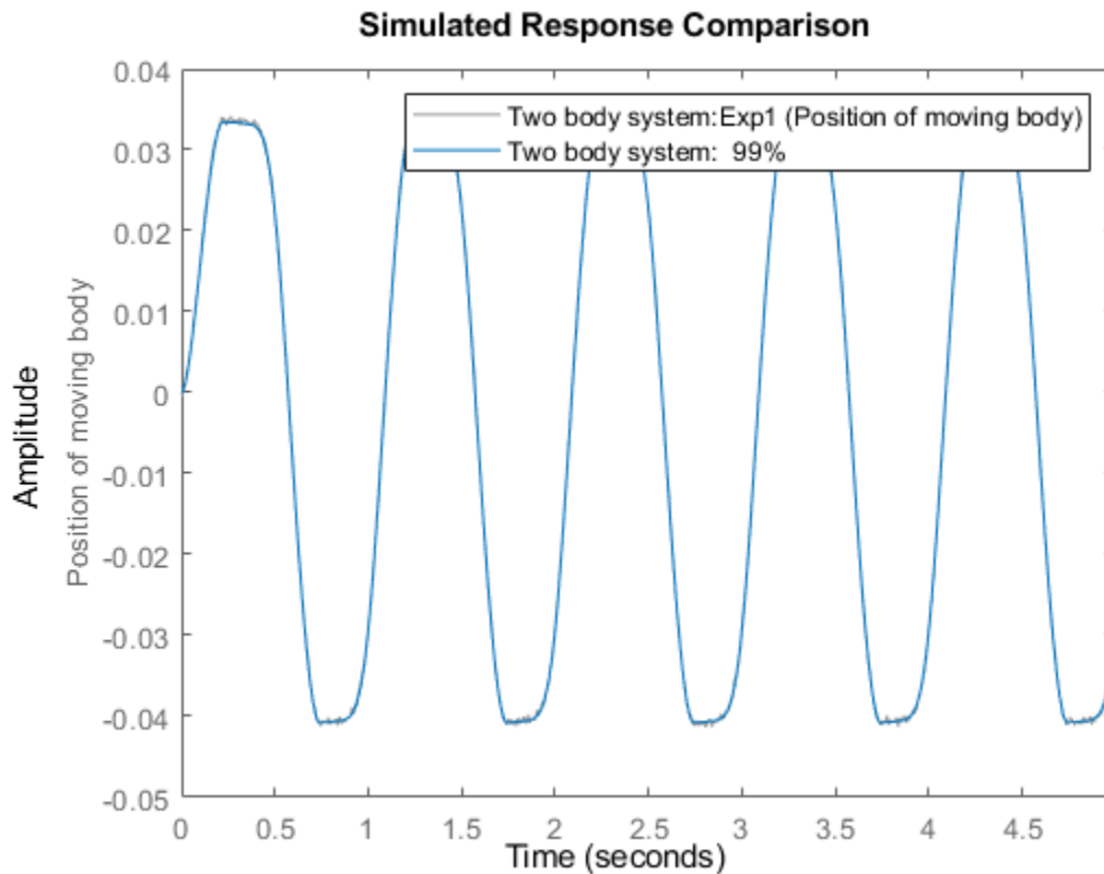
Figure 4: Comparison between true outputs and the simulated outputs of the estimated two body model.
