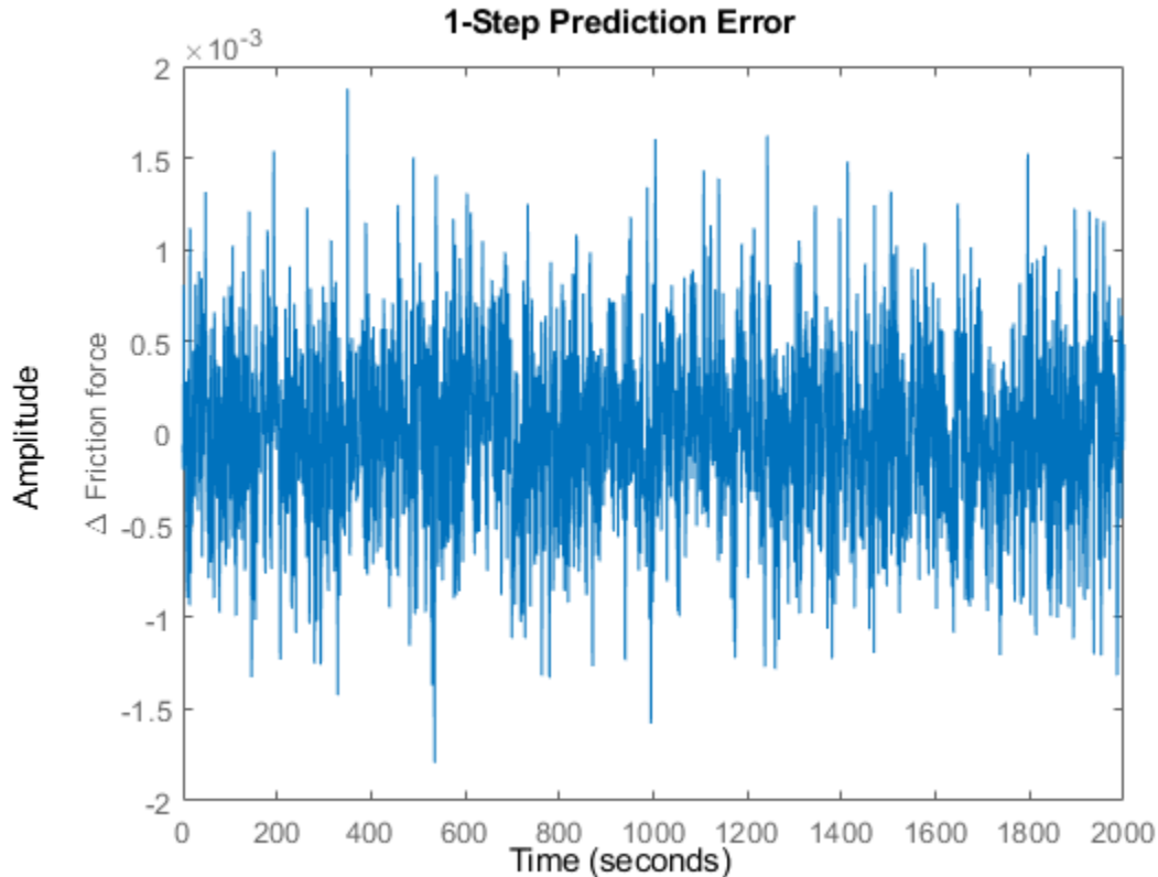
Figure 4: Prediction errors obtained with the estimated full friction model.
