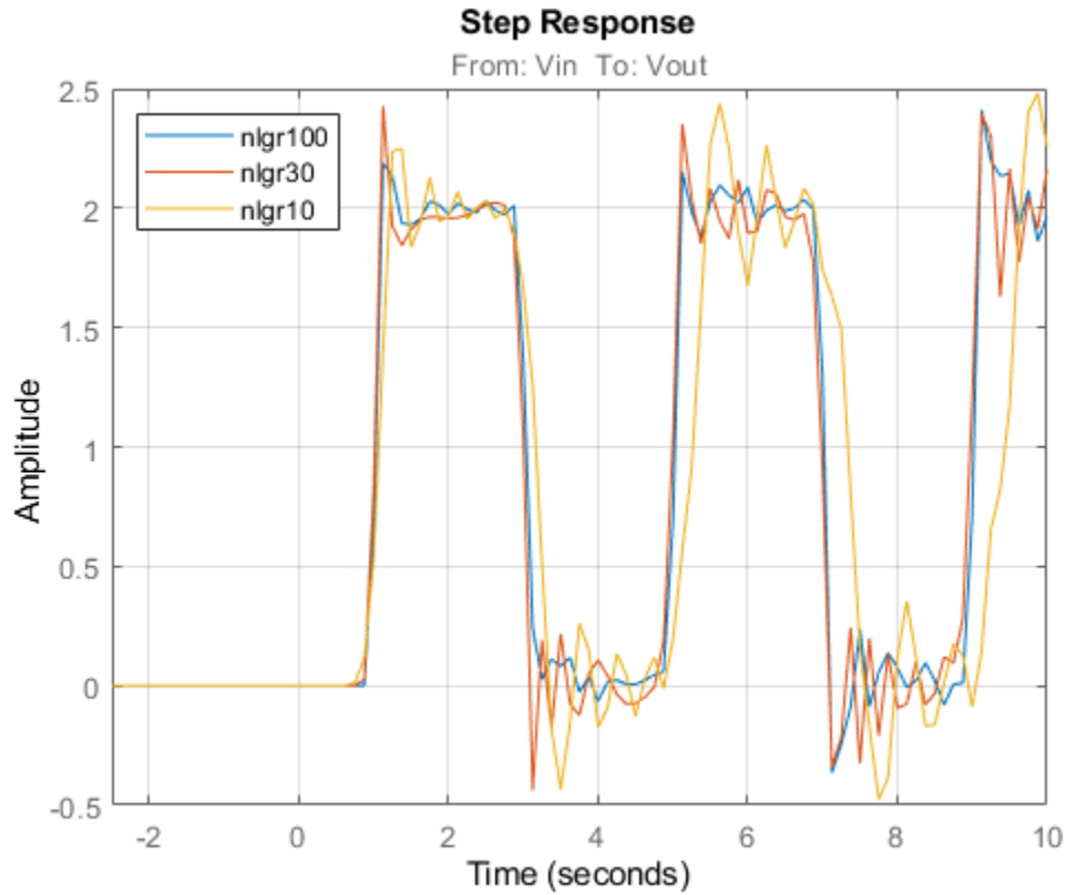
Figure 7: Step responses of three estimated IDNLGREY signal transmission models.
