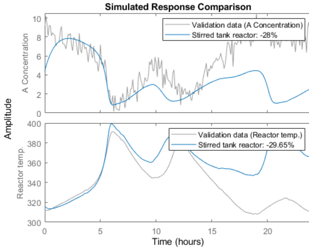
Figure 4: Comparison between the true outputs and the simulated outputs of the initial CSTR model.
